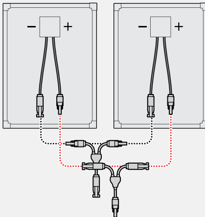
Figure 2.8.1.1: Connecting solar panels in parallel
