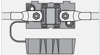
Figure 2.6.1: MIDI style bolt-down fuse
