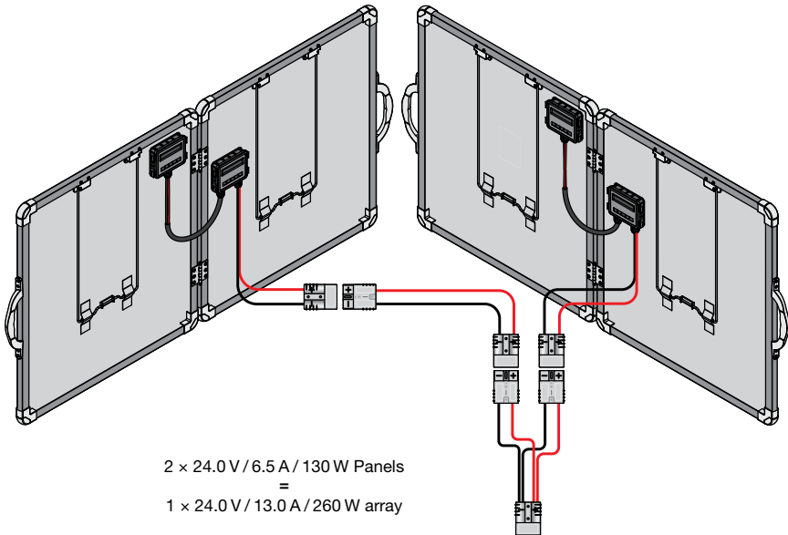
Parallel Connection
